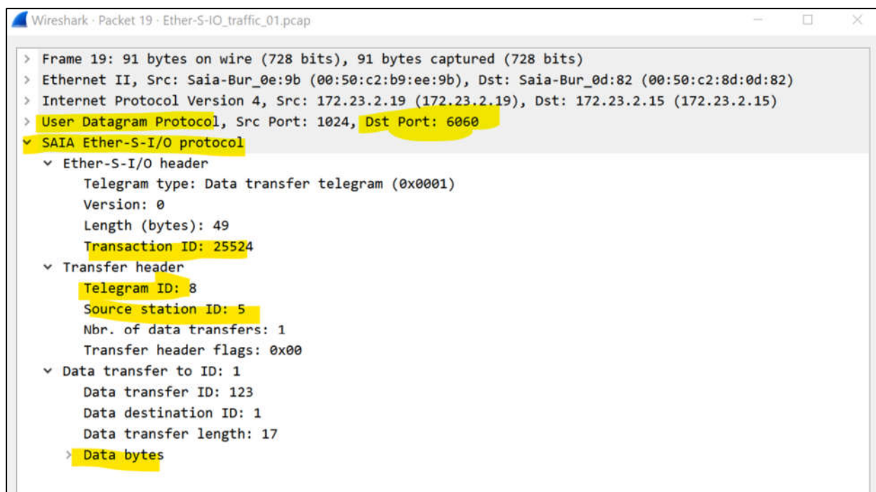
Figure 14. Ether-S-I/O Packet Example [22].
